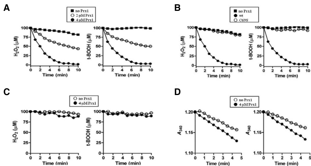
Fig. 2. Peroxidase activity of Prx1. Mean values of triplicate experiments are shown. (A) DTT-dependent removal of H 2 O 2 (left panel) and t-BOOH (right panel) by Prx1. Peroxidase reaction was carried out at room temperature in 200 μl of reaction mixture containing 50 mM HEPES (pH 7.0), 5 mM DTT, 100 μM H 2 O 2 or 100 μM t-BOOH, and in the absence (closed square) or presence of Prx1 (closed circle, 2 μM; closed triangle, 4 μM). At the indicated times, the remaining peroxides were measured using FOX1 reagent as described in Materials and methods. (B) Peroxidase reaction was carried as in (A) with 100 μM H 2 O 2 (left panel) or 100 μM t-BOOH (right panel) in the absence (closed square) or presence of 4 μM Prx1 (wild type, closed circle; C69S, closed triangle). (C) Peroxidase reaction was performed using 4 μM Prx1 as in (A), except the presence of GSH instead of DTT as a reducing equivalent: closed square, without Prx1; closed triangle, with Prx1. (D) Peroxidase activity linked to NADPH oxidation with S. cerevisiae Trx system was monitored by decreases of A 340 in a 200-μl reaction mixture containing 50 mM HEPES (pH 7.0), 0.2 mM NADPH, 2 μM ScTrr1, 5 μM ScTrx1, 4 μM Prx1, and either 0.1 mM H 2 O 2 (left panel) or 0.1 mM t-BOOH (right panel): closed square, without Prx1; closed triangle, with Prx1.
